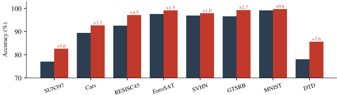
RegMean++ E2E (ours) Per-task accuracy, CLIP ViT-L/14 (8-task merge)
